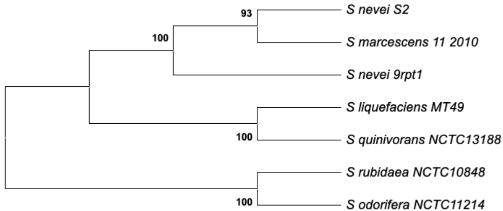
Fig. 1. Phylogenetic analyses applied to the evolutionary history of Serratia sp. pst operon
