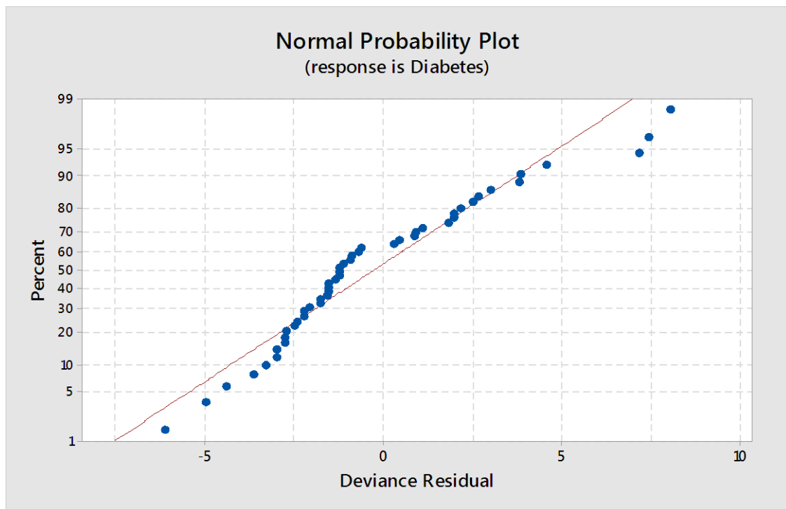
Fig. 1. Normal probability plot
