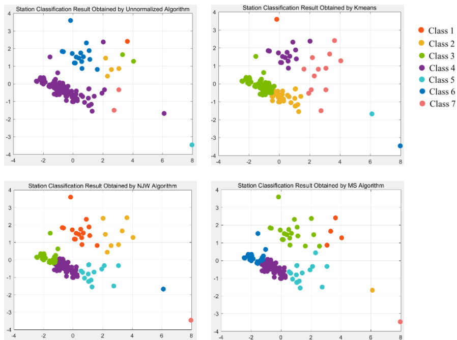
Fig. 3. Station classification result obtained by different clustering methods
