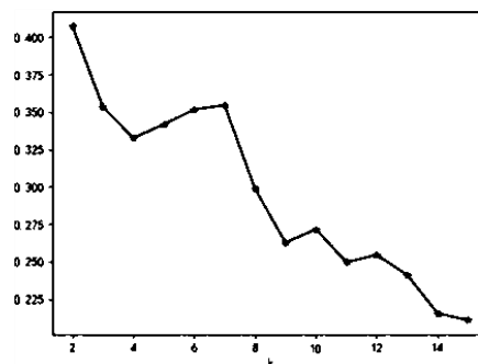
Fig. 1. The relationship between k and the Silhouette Coefficient
