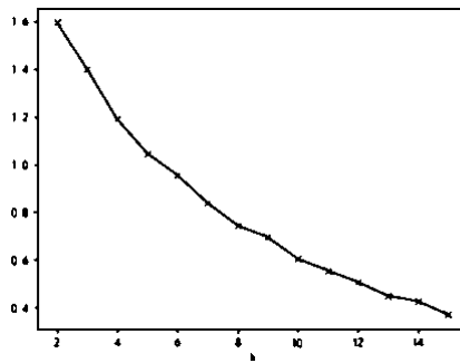
Fig. 2. The relationship between k and SSE
