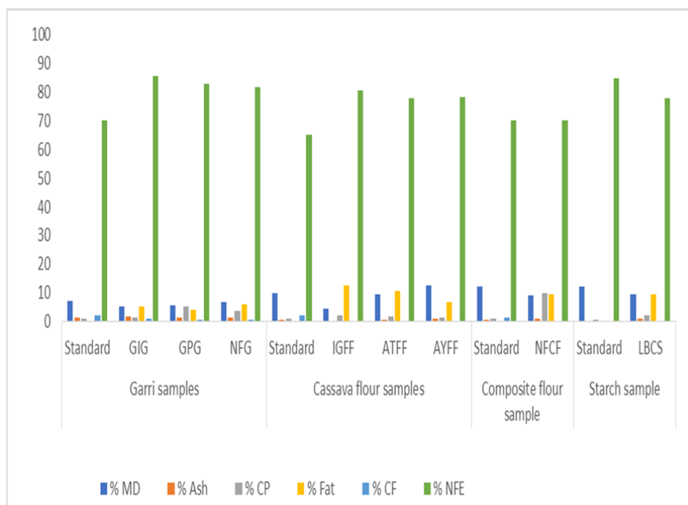
Fig. 2. Proximate composition of the eight processed cassava products
