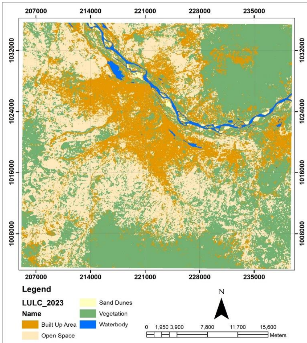
Fig. 3. Landcover/landuse map of Greater Yola 2023
