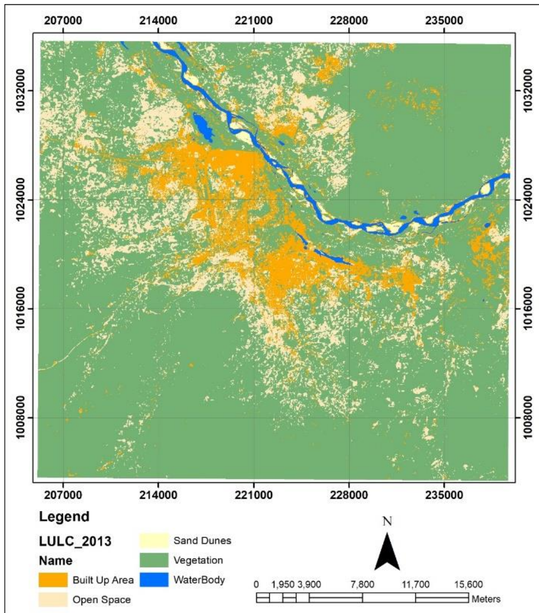
Fig. 1. Landcover/landuse map of Greater Yola in 2013
