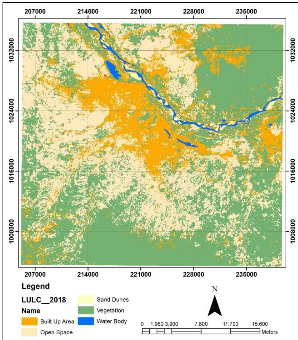
Fig. 2. Landcover/landuse map of Greater Yola in 2018
