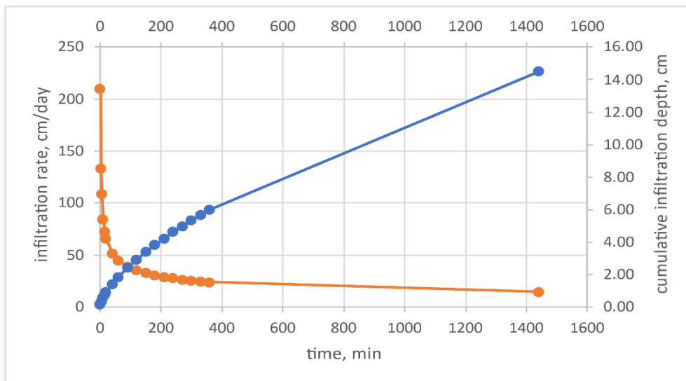
Fig. 4. Measured values of infiltration rate and K_s by infiltrometer test
