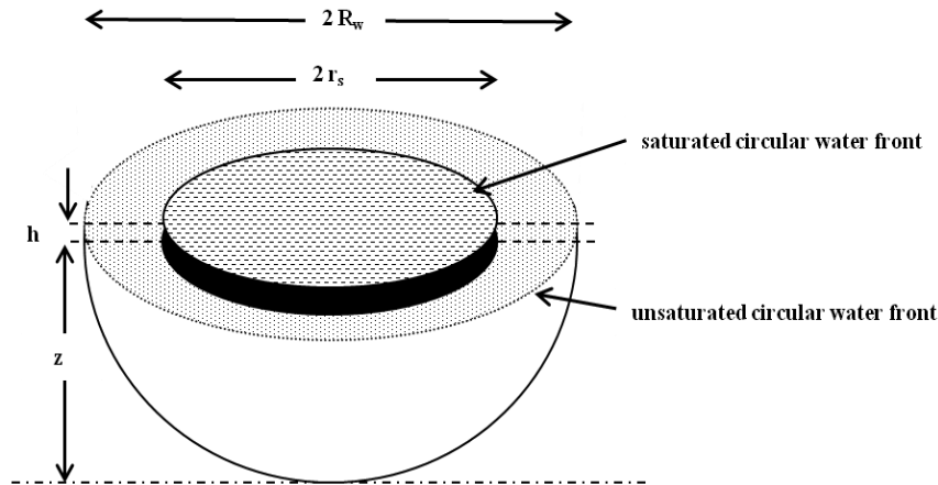
Fig. 1. Water flow geometry under shallow circular pond over soil surface
