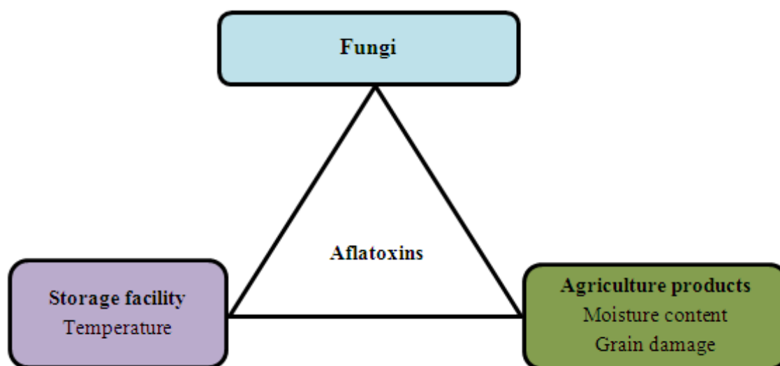
Fig. 1. Cycle for synthesis of aflatoxins
