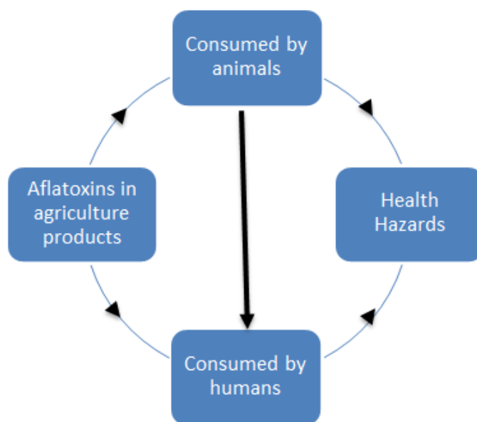
Fig. 3. Aflatoxins flow along the feeding cycle leading to health
