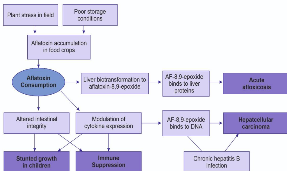
Fig. 5. Aflatoxins disease pathway in humans
