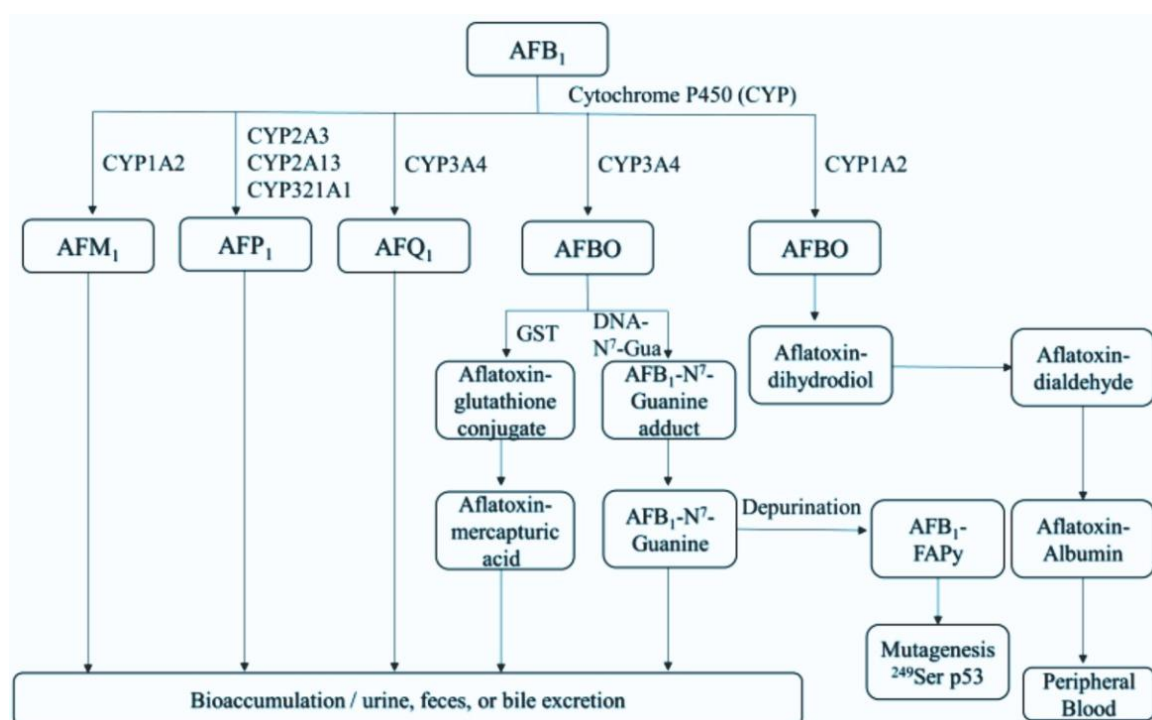
Fig. 4. Overview of AFB1 metabolism and excretion in humans and animals
