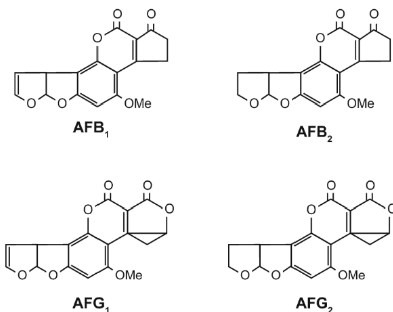
Fig. 2. Structures for the types of aflatoxins
