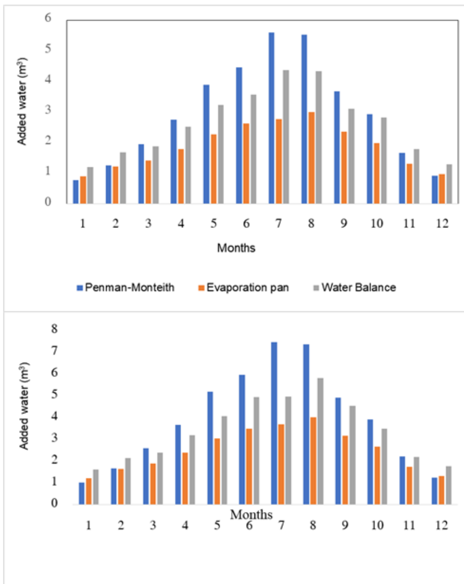
Fig. 2. Monthly water requirements calculated using different equations.
