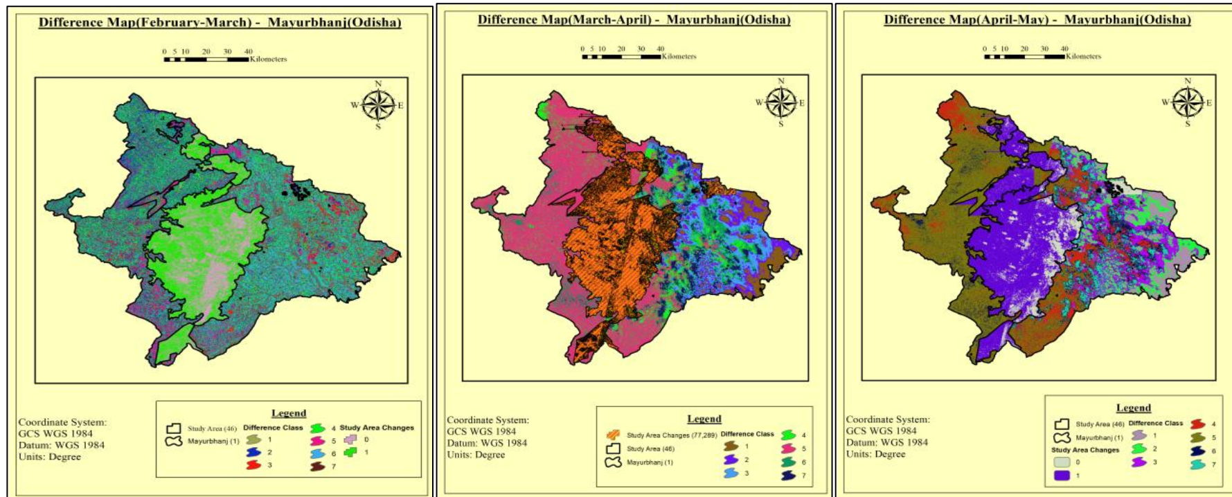
Fig. 5. The changes in land cover of Mayurbhanj during Feb.-Mar, Mar-Apr and Apr-May-2021
