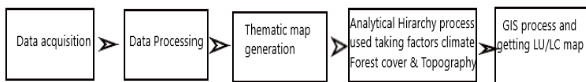
Fig. 1. Methodology used for spatial analysis of the Similipal wild fire hazard in 2021
