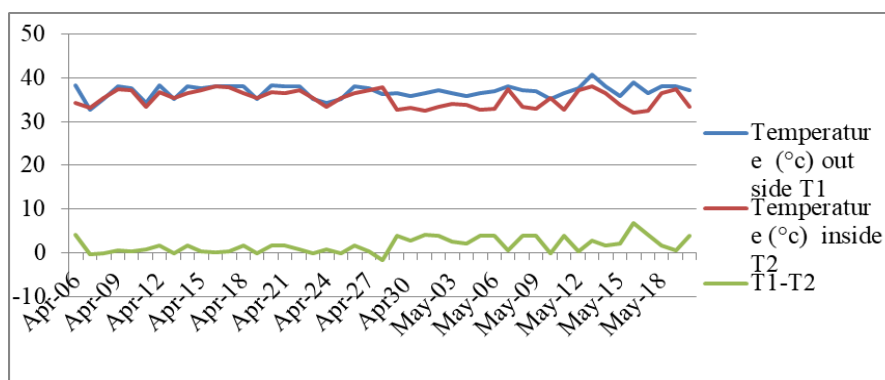
Fig. 3. Variation of temperature inside and outside of polyhouse at 08:30 Am
