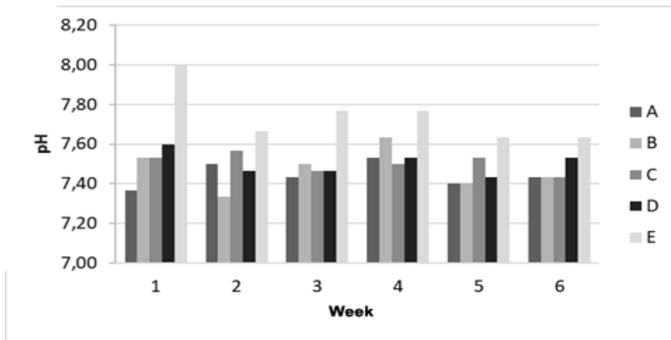
Fig. 9. Results of the average pH
