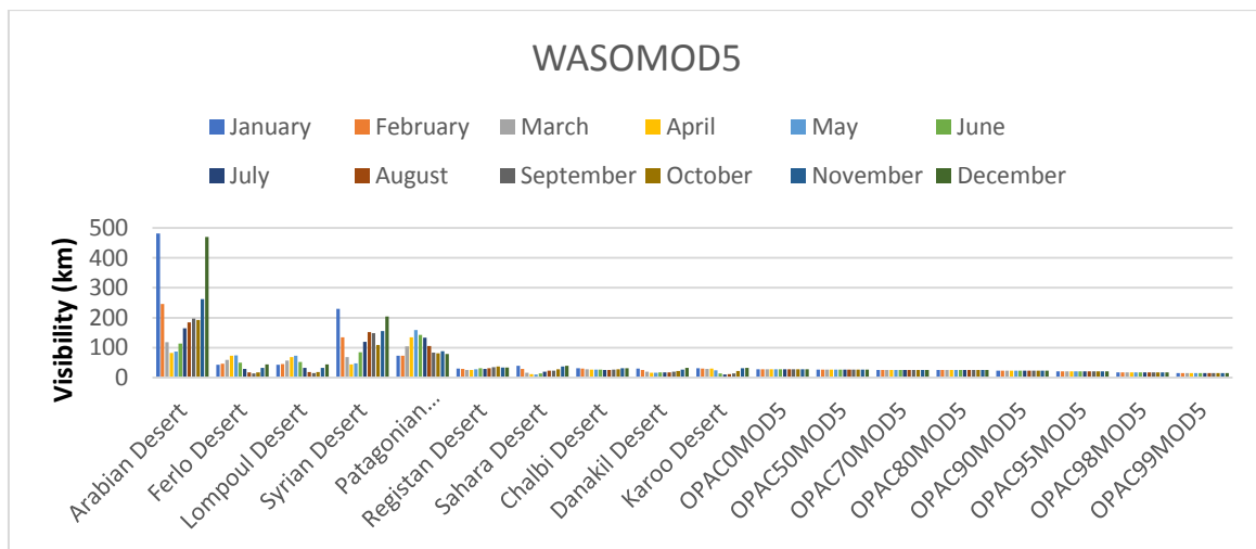
Fig.1b. Visibility plot for OPAC and MEERA-2 (WASO Model5) at 550nm
