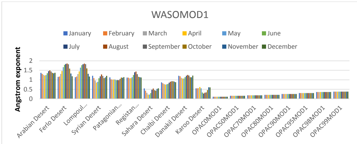
Fig. 2a. Angstrom exponent plot for OPAC and MEERA-2 (Model1) at 550nm
