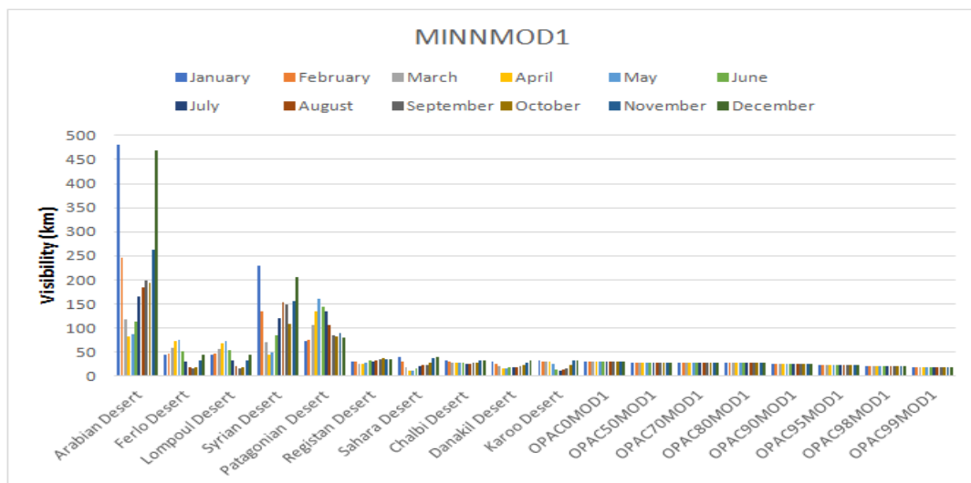
Fig. 1c. Visibility plot for OPAC and MEERA-2 (MINN Model1) at 550nm
