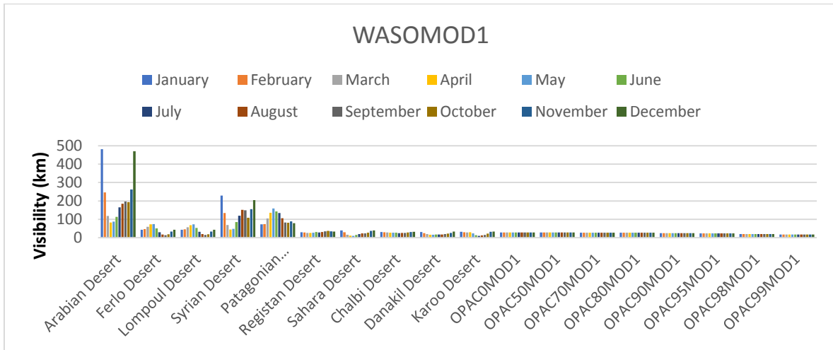
Fig. 1a. Visibility plot for OPAC and MEERA-2 (WASO Model1) at 550nm
