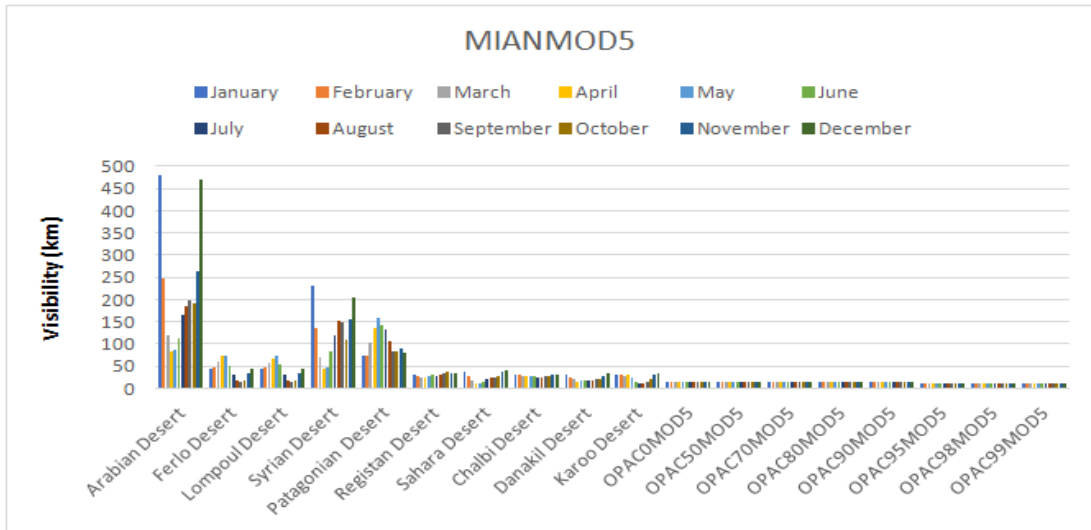
Fig. 1f. Visibility plot for OPAC and MEERA-2 (Model5) at 550nm
