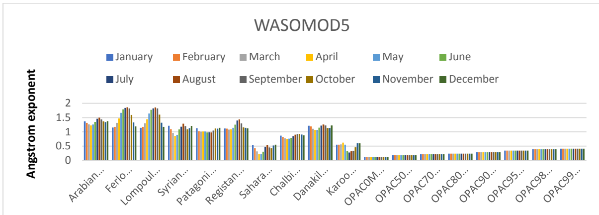
Fig. 2b. Angstrom exponent plot for OPAC and MEERA-2 (Model5) at 550nm
