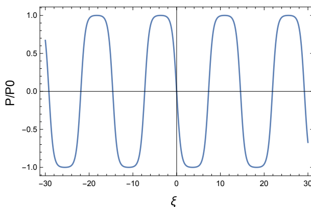
Fig. 1. Periodic domain wall solution of the \phi^4 equation
