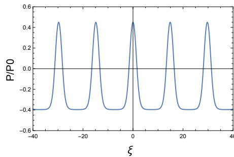
Fig. 2. Periodic domain wall in the presence of an external field
