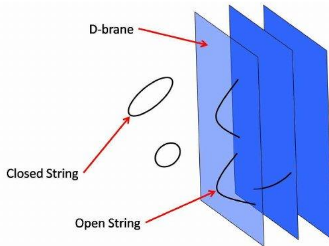
Fig. 2. Closed strings with no boundary attachments to Branes, hence allowed to move in extra-spacial dimensions. Whereas, open strings being attached to Branes couldn't make inter-dimensional travel and are restricted to oscillating in present dimensions. Those Branes which have a 'radion' fields in them, when contracts then, touches each other making a high explosion giving birth to a new universe, while when they start to move away from each other, then the universe expands which this cycles of Branes getting away from each other, and again coming close to each other is expressed via the 'cyclic cosmology' or 'Ekpyrotic cosmology'. The standard model of particle physics resides in the Branes while the gravity being closed strings are free from any dimensional confinements. Dimensions are there in Branes which remain floating in the Bulks. [Image courtesy: Myers, R. C., and Vázquez, S. E. (2008). Quark soup al dente: applied superstring theory. Classical and Quantum Gravity , 25(11), 114008. https://doi.org/10.1088/0264-9381/25/11/114008 ]
