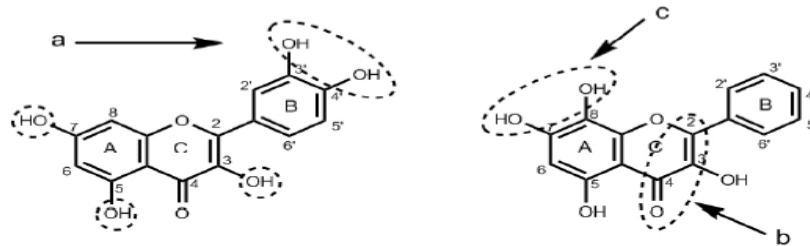
Fig. 3. The flavonoid structure-antioxidant activity relationships
