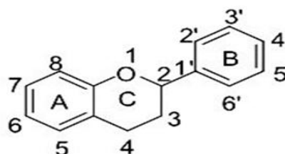
Fig. 2. Basic structure of flavonoids (Phenylbenzopyrane)
