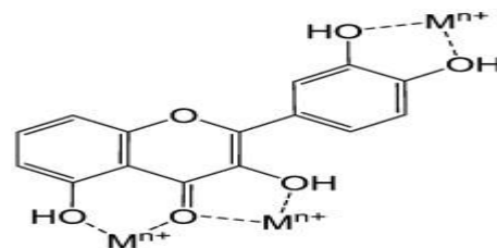
Fig. 5. Binding sites for trace metals [117]
