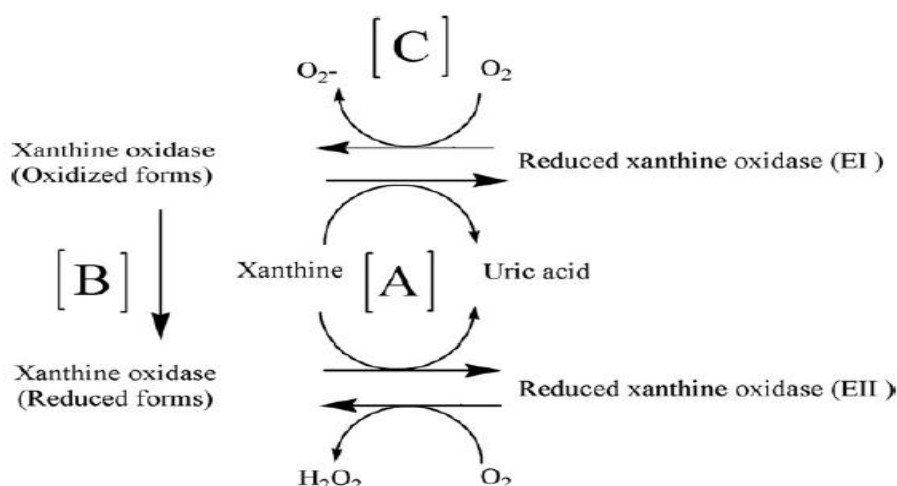
Fig. 6. The inhibition of the superoxide anion generation catalyzed by xanthine oxidase with antioxidants consisted of three reactions (A, B and C). [A] Inhibition of the xanthine oxidase reaction with antioxidants. [B] Reduction of the xanthine oxidase with antioxidants. [C] Scavenging of the superoxide anion with antioxidants [120]
