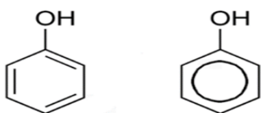
Fig. 1. Phenol, the most straightforward component of phenolic compounds
