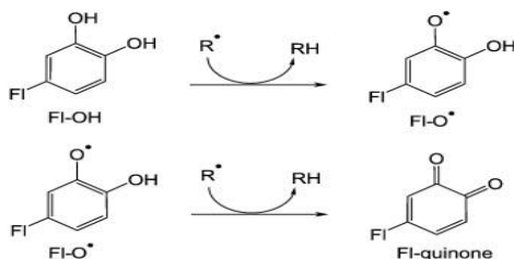
Fig. 4 Scavenging of reactive oxygen species ( \text{R}^\bullet ) by flavonoid. The free radical \text{FI-O}^\bullet may react with a second radical, acquiring a stable quinone structure [117]
