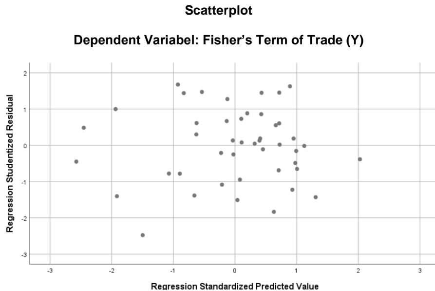
Fig. 2. Fisher heteroscedasticity
