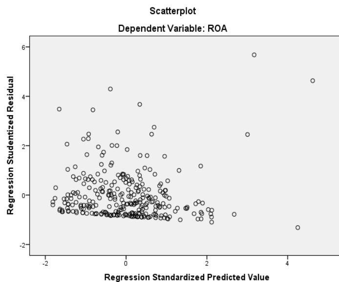
Fig. 4. Heteroscedasticity test results-equation 1
