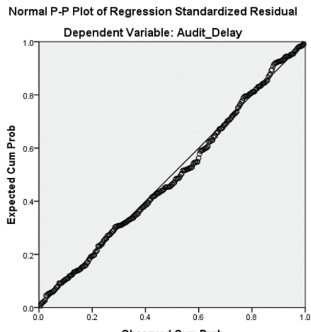
Fig. 3. Normality test results-equation 2 Source: Processed secondary data (2021)
