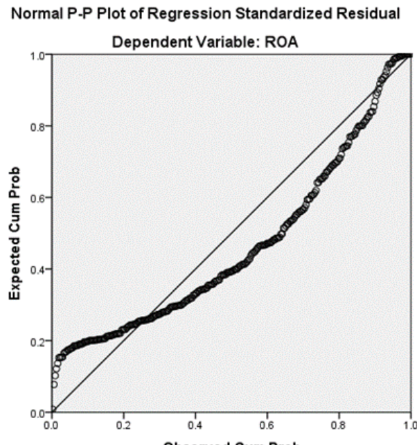
Fig. 2. Normality test results-equation 1 Source: Processed secondary data (2021)
