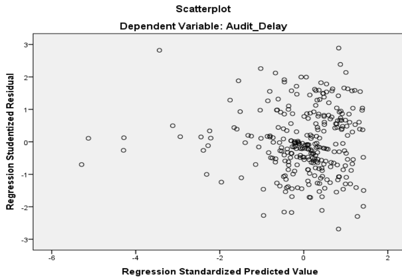
Fig. 5. Heteroscedasticity test results-equation 2
