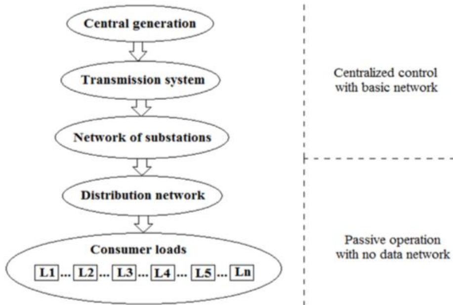
Fig. 4. Existing electricity utility grid
