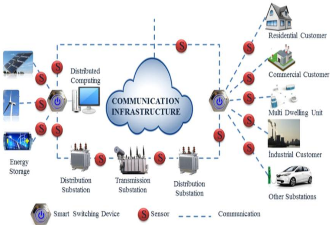
Fig. 3. Smart grid architecture increases the capacity and flexibility of the network and provides advanced modern communications technologies through sensing and control
