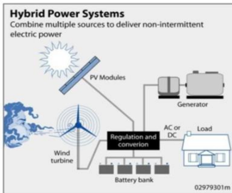
Fig. 6. Hybrid power system
