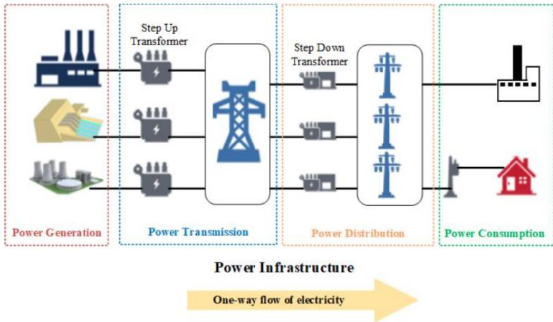
Fig. 2. Structure of classical power grid
