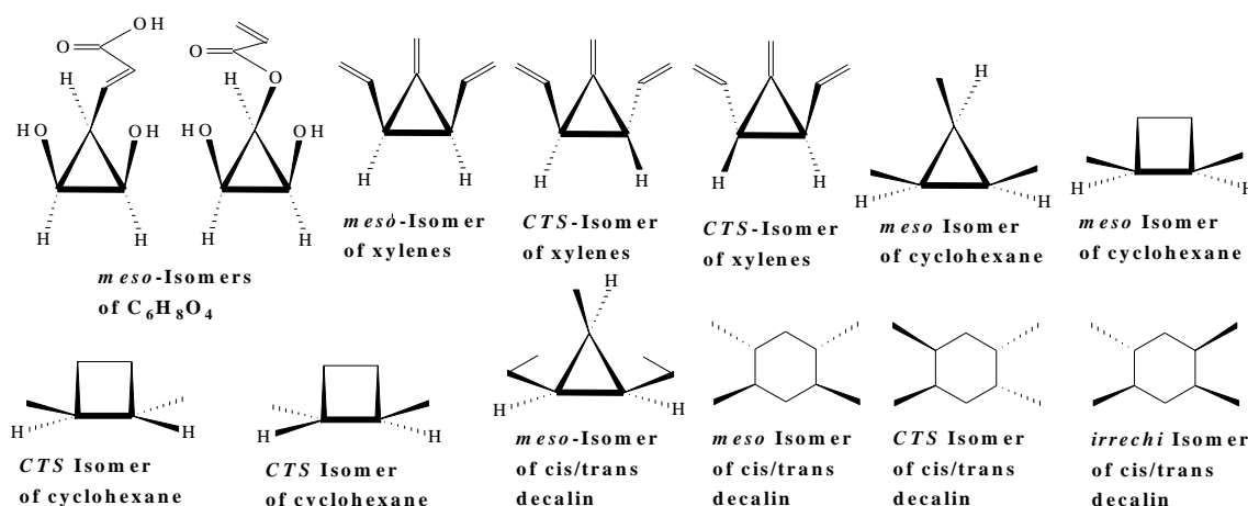
Fig. 1. Meso isomers of unsaturated (fumaric/maleic acid), aromatic, and the latter's saturated compounds
