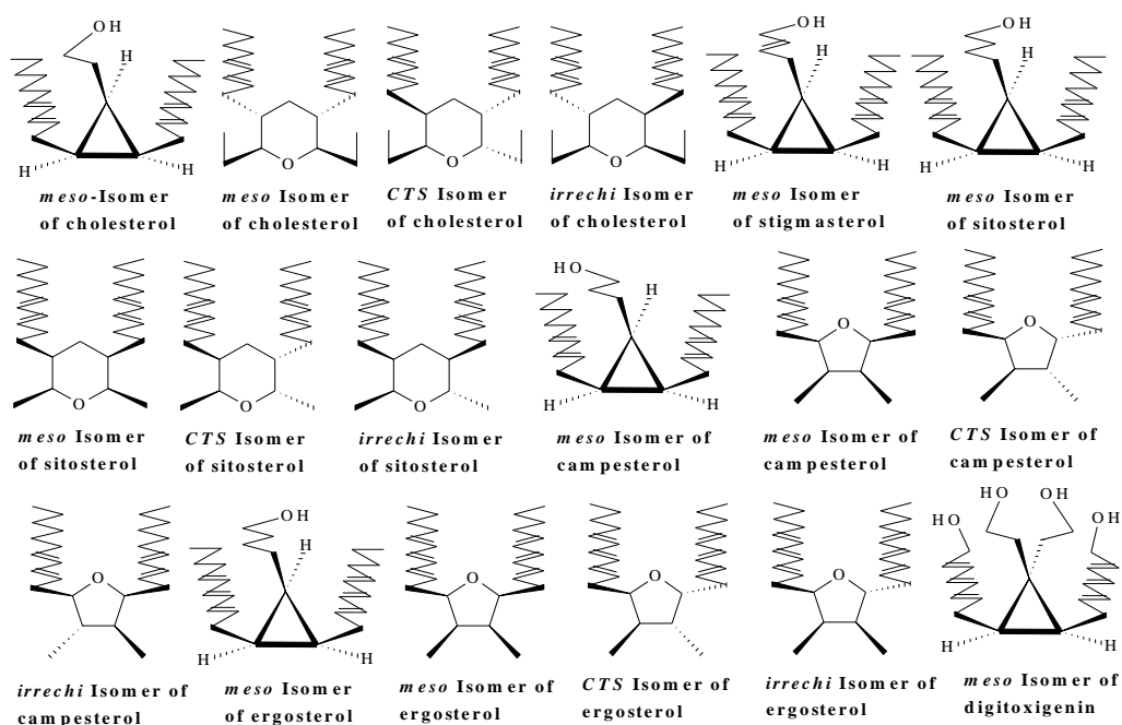
Fig. 9. Meso isomers of some natural sterols
