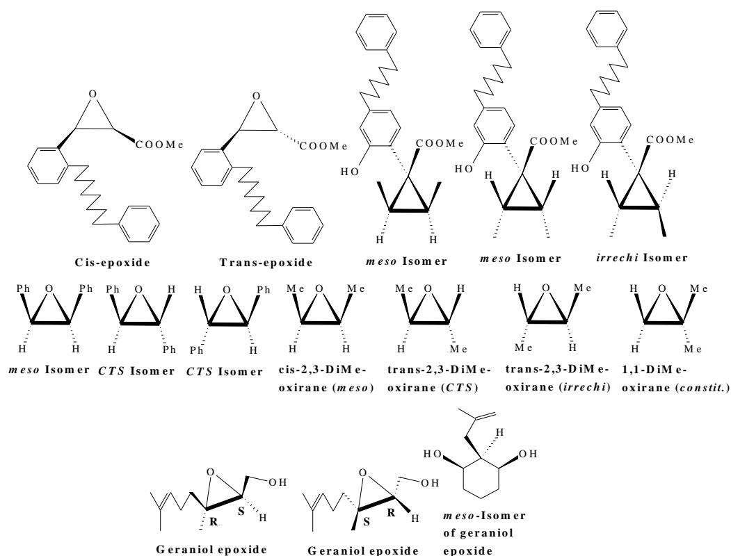
Fig. 4. Meso isomers of some epoxides
