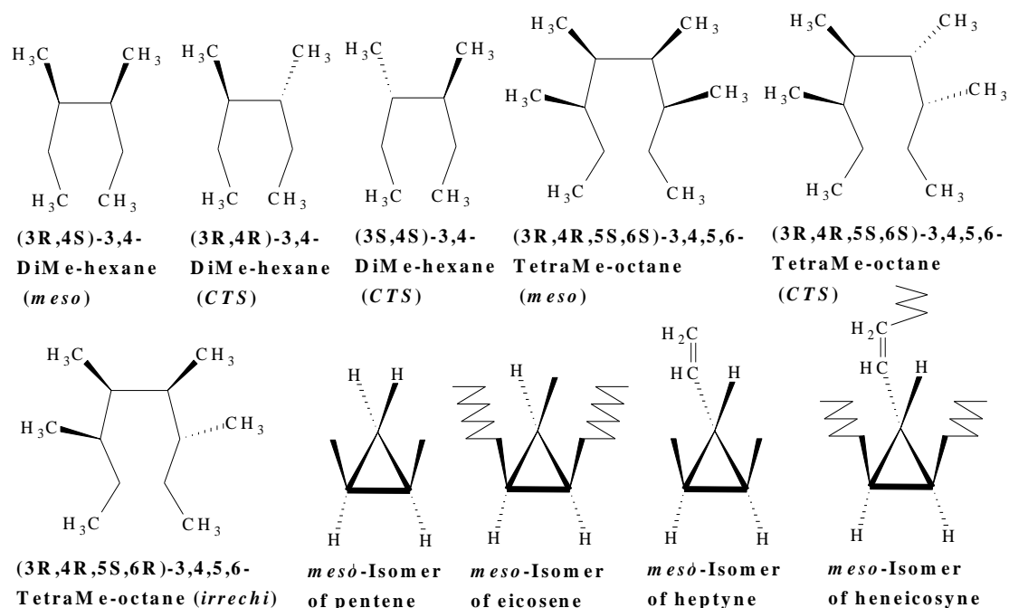
Fig. 2. Meso isomers of saturated and unsaturated hydrocarbons
