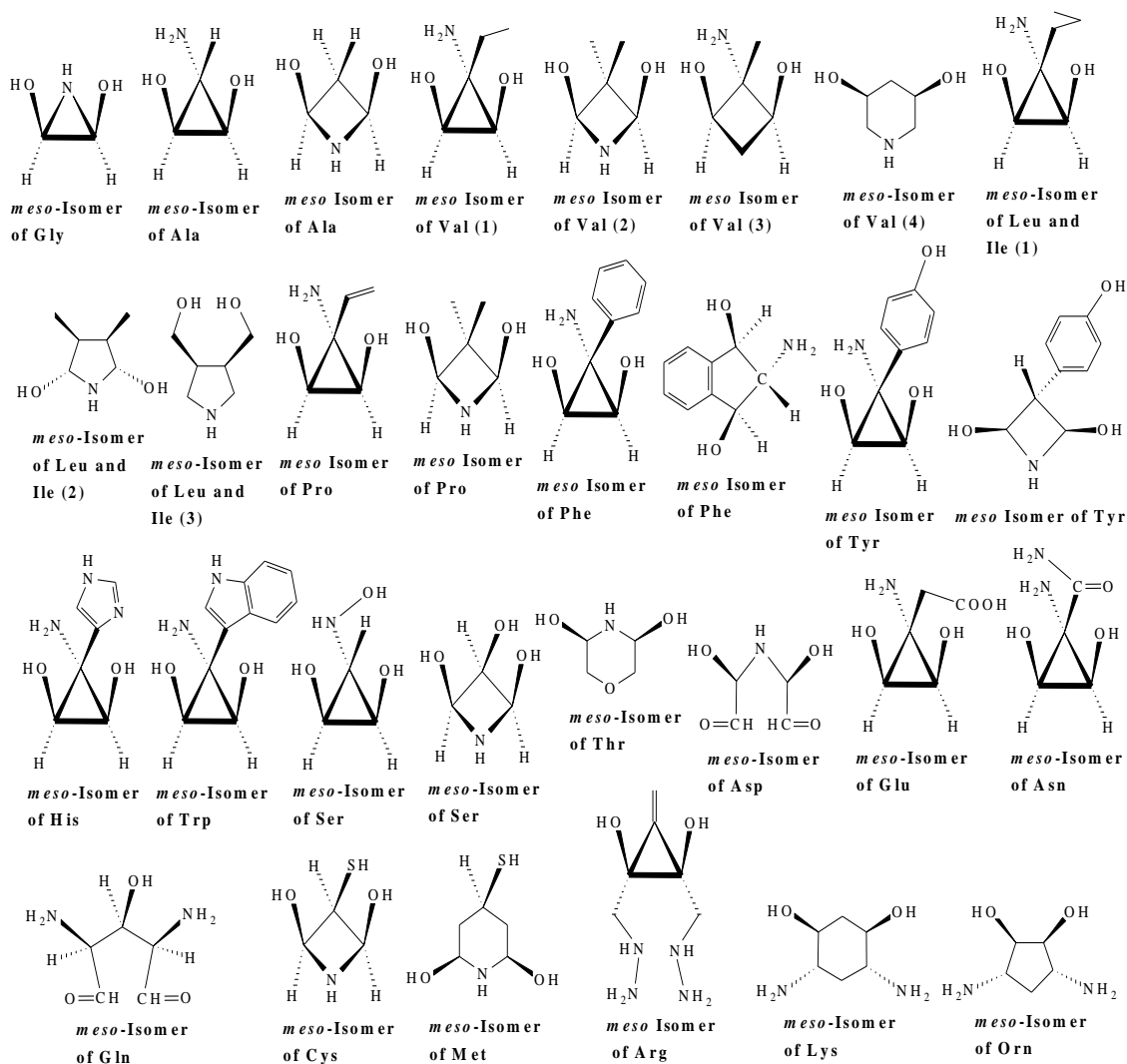
Fig. 7. Meso isomers of the twenty fundamental amino acids. (see also text)
