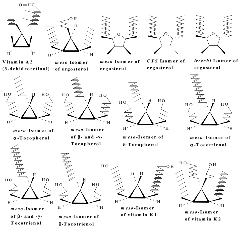
Fig. 10. Meso isomers of lipophilic vitamins
