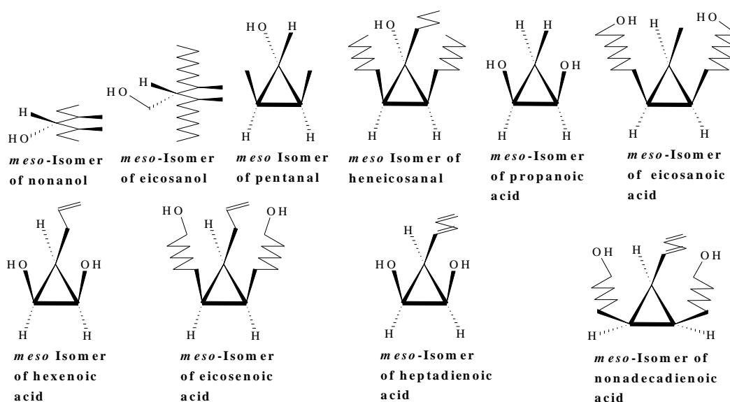
Fig. 3. Meso isomers of some serial compounds with functional groups
