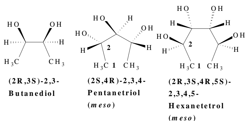
Fig. 5. Meso isomers of diols, triols, tetrols
