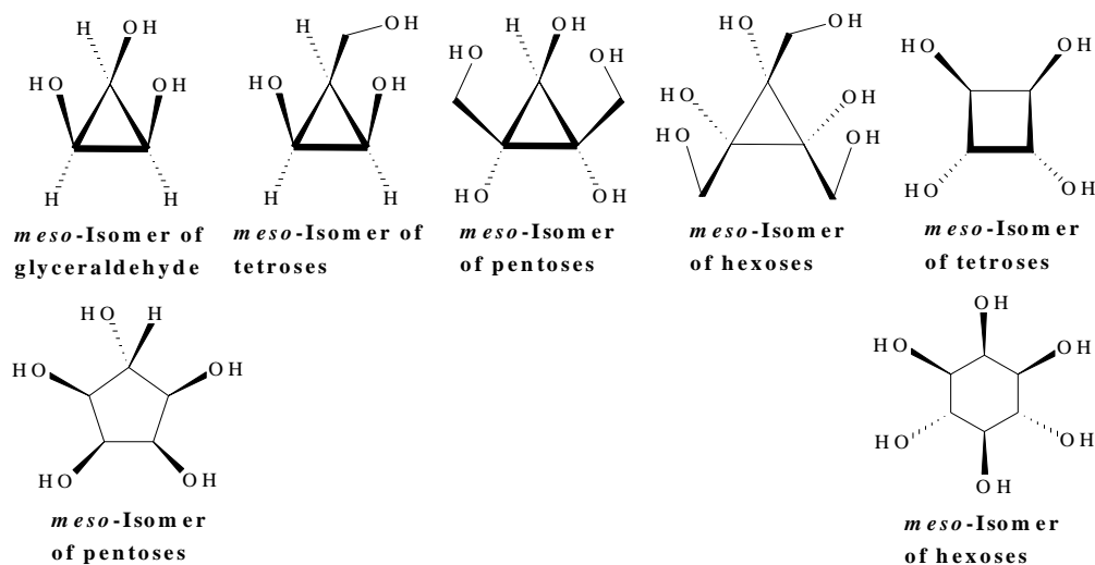
Fig. 6. Meso isomers of aldoses and ketoses
