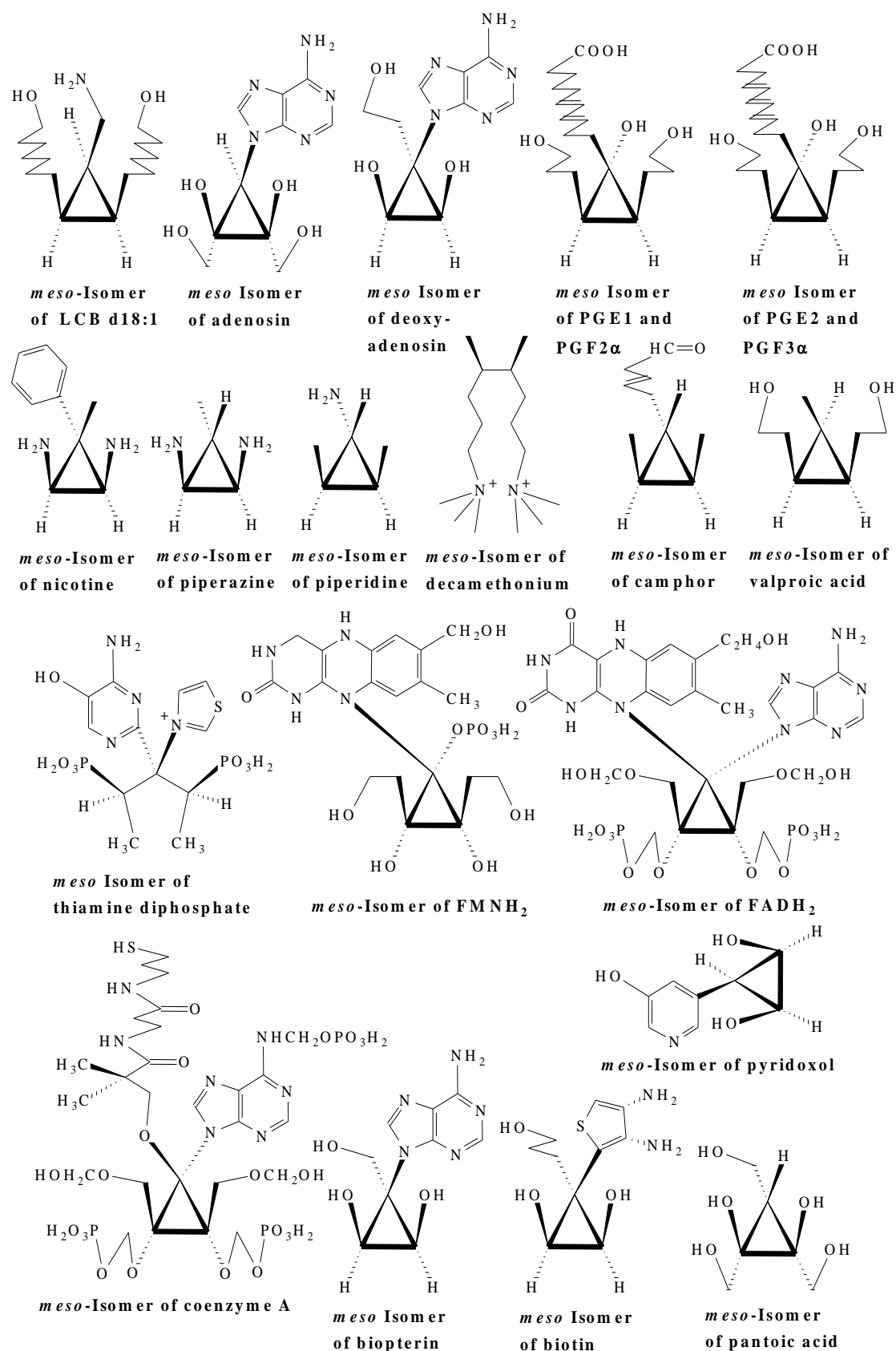
Fig. 8. Meso isomers of some natural compounds, including hydro-soluble vitamins
