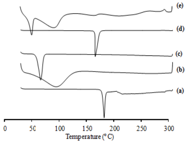
Fig. 2. DSC Thermograms of (A) GLB, (B) HPMC, (C) PEG-8000, (D) NA-CITRATE AND (E) GCHP-4
