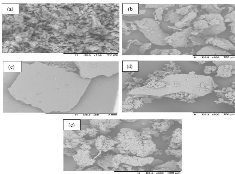
Fig. 5. SEM images of (a) GLB, (b) HPMC, (c) PEG-8000, (d) Na-citrate and (e) GCHP-4
