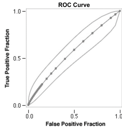
Fig. 2. ROC curve qSOFA \geq 2 score in predicting ICU mortality showing AUC 0.56; 95% CI 0.46-0.66
