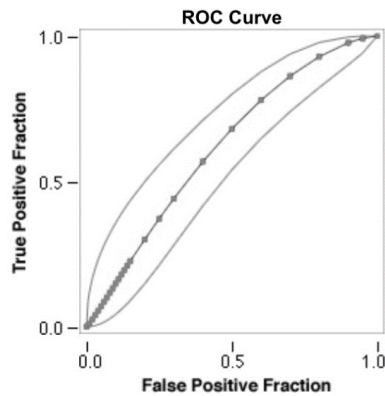
Fig. 3. ROC curve NEWS \geq 5 score in predicting ICU mortality showing AUC 0.61; 95% CI 0.52-0.71
