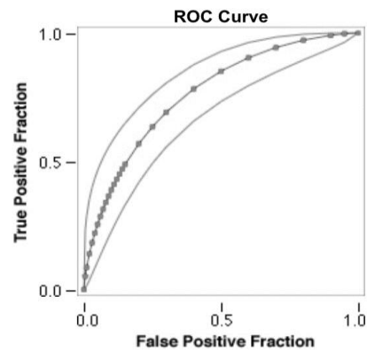
Fig. 4. ROC curve MEWS \geq 5 score in predicting ICU mortality showing AUC 0.76; 95 % CI 0.68-0.84
