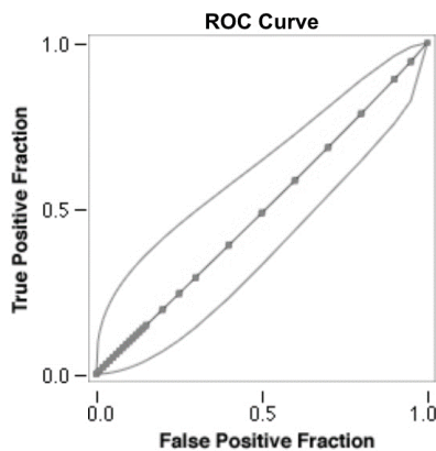
Fig. 1. ROC curve SIRS \geq 2 score in predicting ICU mortality showing AUC 0.49; 95% CI 0.37-0.61
