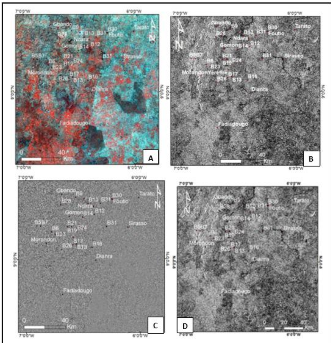
Fig. 3. Landsat 8 OLI image and radar image processing. (A): Color-coded (567) OLI image; (B): Image filtered by Gaussian high pass filter applied on band 8 of OLI image; (C): Radar SAT image; (D): Radar ERS image (negative print)
