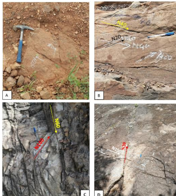
Fig. 9. (A): Outcrop of fractured metasediments with intersecting fractures; (B): Outcrop of diorite affected by the N20° fractures intersecting the N40° fractures in dextral shear; (C): Folded metasediments presenting fractured networks, the N160° networks intersect the N60° networks; (D): Outcrop of fractured gneiss with N150° fractures intersecting the N20° fractures
