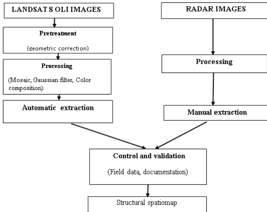
Fig. 2. Landsat 8 image and radar images processing methodology
