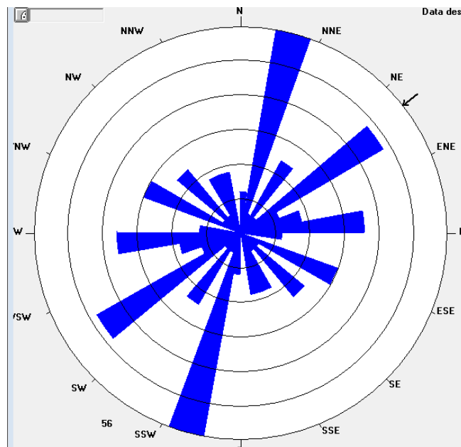
Fig. 8. Directional rose of the fractures in the study area
