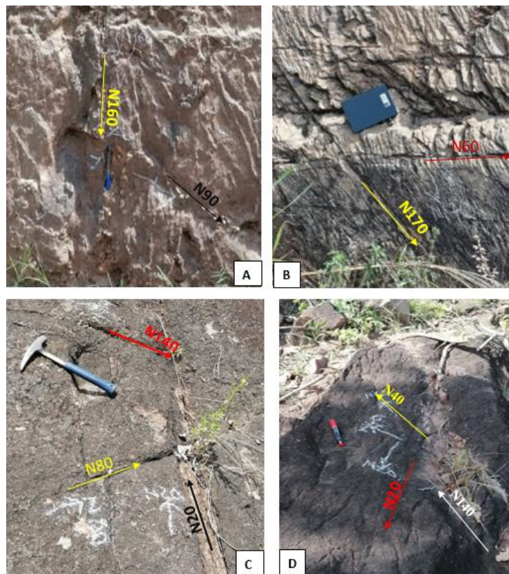
Fig. 10. Lithological and structural data about some of the outcrops in the study area. (A) : Outcrop of metasediments in which the N160 quartz veins intersect the N90° veins (B) : Fractured metasediment with N170° and N60° fractures intersecting; (C) : Fractured biotite granite outcrop, the N20° fractures are intersected by the N140° fractures and both fracture networks are intersected by N80° fractures; (D): Fractured biotite granite outcrop with directions: N20° intersected by N140°, N40° intersected by N20°
