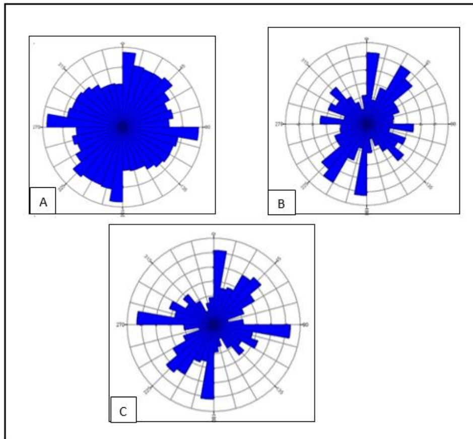
Fig. 7. Directional statistical analysis. (A): Rose diagram of the lineaments extracted automatically; (B): Rose diagram of the lineaments extracted manually from radar Sat image; (C): Rose diagram of the lineaments extracted manually from radar ERS image
