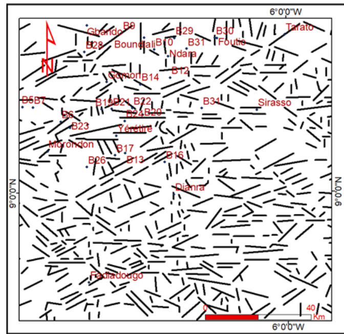
Fig. 6. Map of the lineaments extracted manually from radar ERS image
