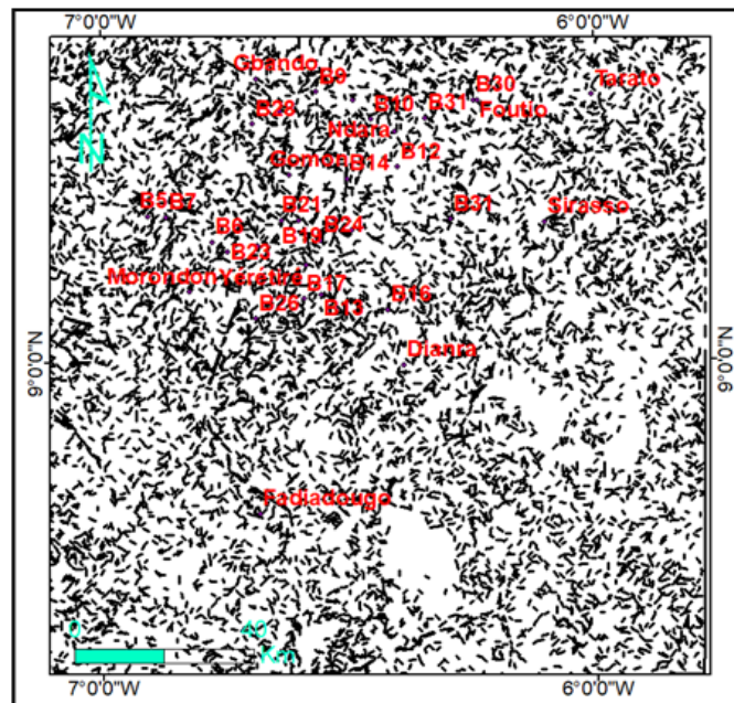
Fig. 4. Map of the automatically detected lineaments
