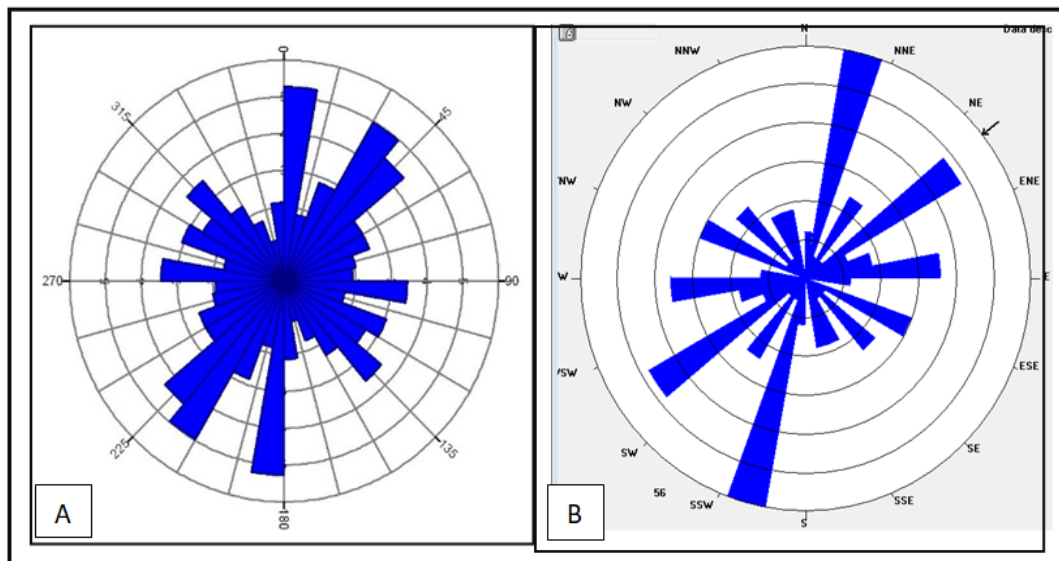
Fig. 11. Comparison of the directional rose diagrams. (A): the lineaments extracted from SAT radar image; (B): field data
