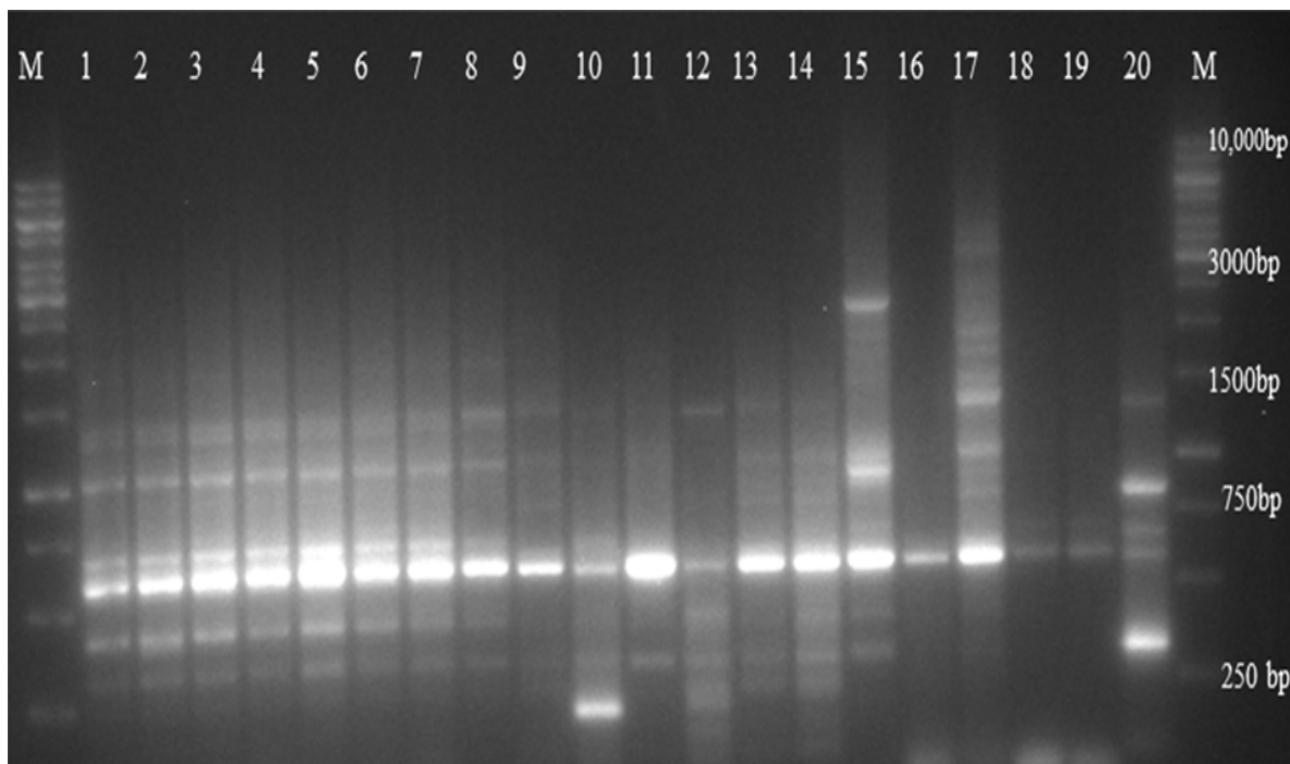
Figure 3. An Example of DNA fingerprint pattern of V. cholerae isolates using the ERIC-PCR. Lane 1-20 is TI58, TI35, TI52, TI23, TI53, BI36, DI20, TI57, BI60, BI42, BI18, BI46, DC47, DC48, DI43, TC63, DC49, BI44, BI34 and TI24, respectively. Lane M: 1 kb DNA Molecular weight maker.
