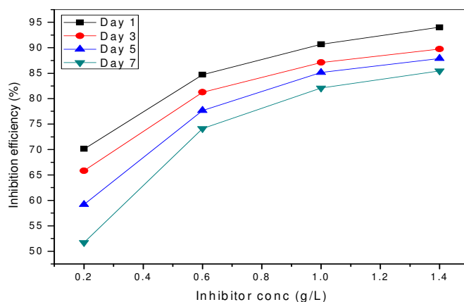
Fig. 1. Variation of inhibition efficiency with different concentrations of MS+KI at room temperature
