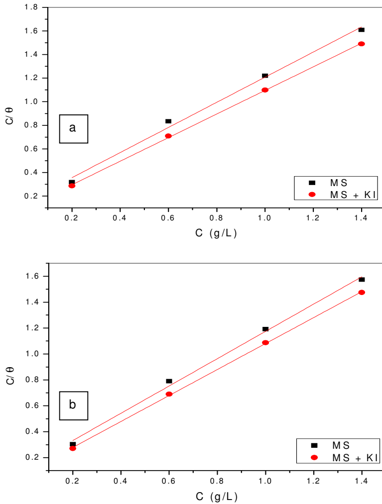
Fig. 2. Plots of Langmuir adsorption isotherms (a) weight loss data and (b) polarization data for the adsorption of millet starch on mild steel in 0.5 M H 2 SO 4
