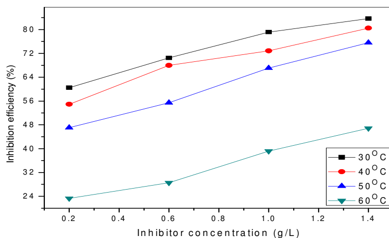
Fig. 3. Variation inhibition efficiency versus inhibitor concentration for mild steel in 0.5 M H 2 SO 4 in the presence different concentrations of MS
