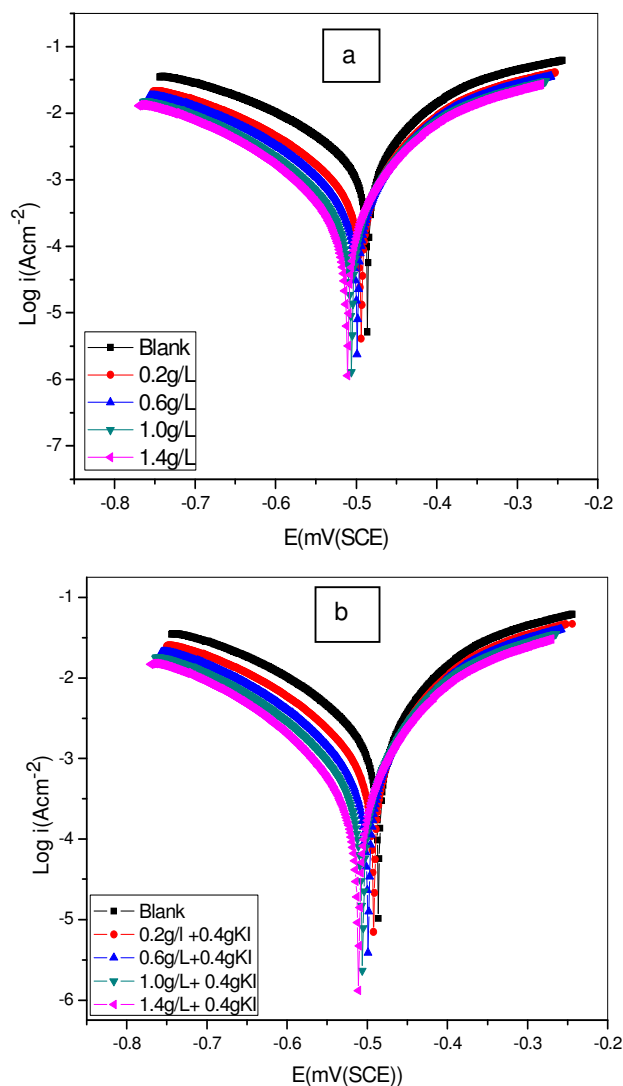
Fig. 6. Polarization curves of mild steel in 0.5 M H 2 SO 4 in the absence and presence of (a) MS and (b) MS+KI
