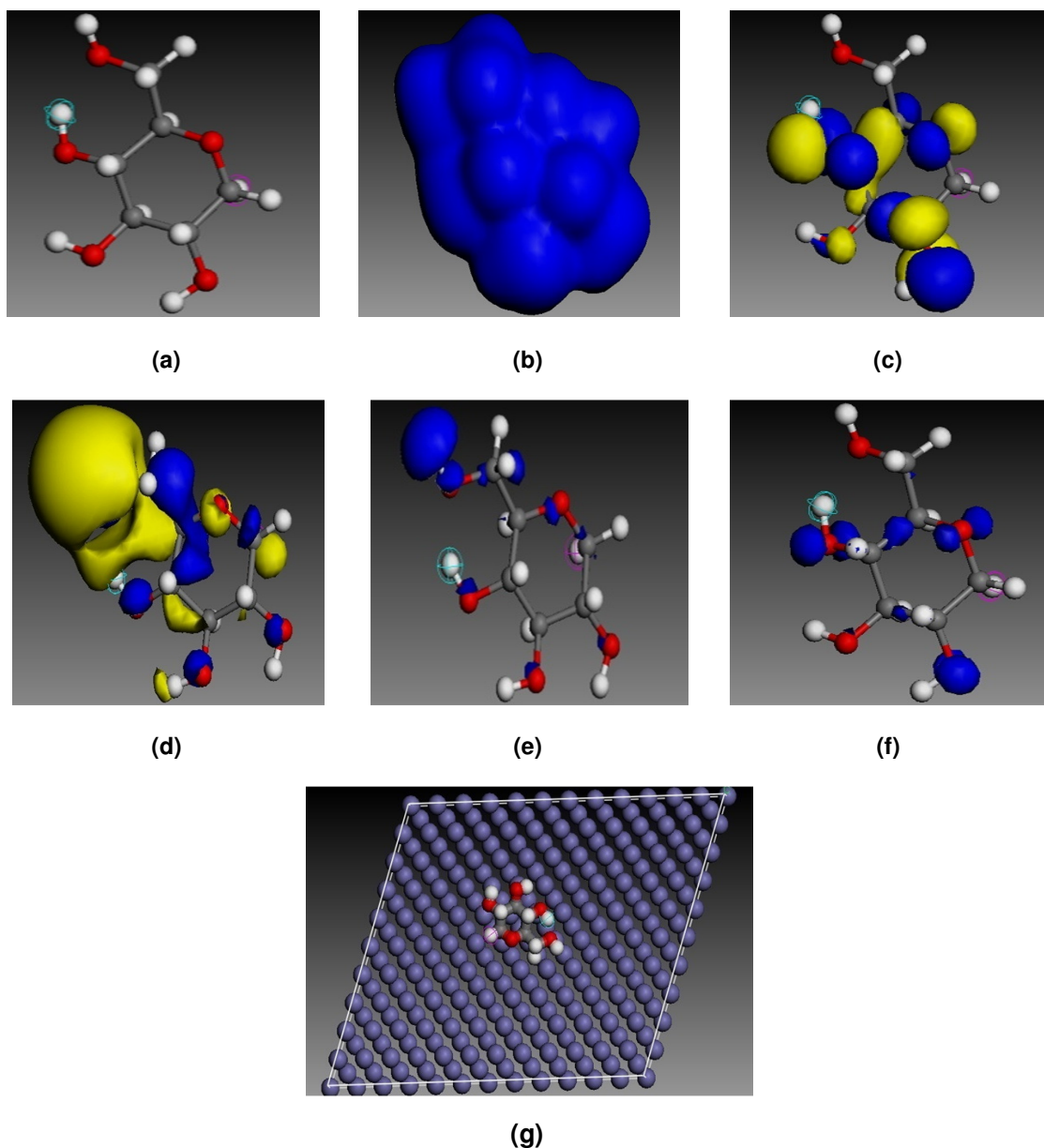
Fig. 7. Electronic properties of glucose unit of starch molecule (a) optimized structure (b) electron density (c) HOMO orbital (d) LUMO orbital, (e) Fukui function for electrophilic attack ( F^- ), (f) Fukui function for nucleophilic attack ( F^+ ) and (g) top view of the lowest energy adsorption orientation for a single glucose molecule on the Fe (110) surface. Atom legend: white = H; gray = C; red = O: The blue and yellow iso-surfaces depict the electron density difference: The blue regions show electron accumulation while the yellow regions show electron loss
