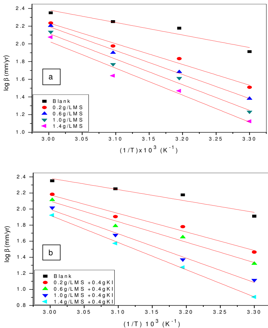
Fig. 4. Arrhenius plots of log ( \beta ) versus 1/T at different concentrations of (a) MS and (b) MS+KI
