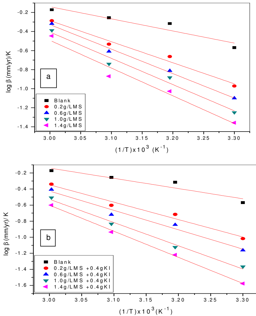
Fig. 5. Plots \log(\beta/T) versus 1/T for mild steel corrosion in 0.5 M H_2SO_4 solution in the absence and presence of (a) MS and (b) MS+KI
