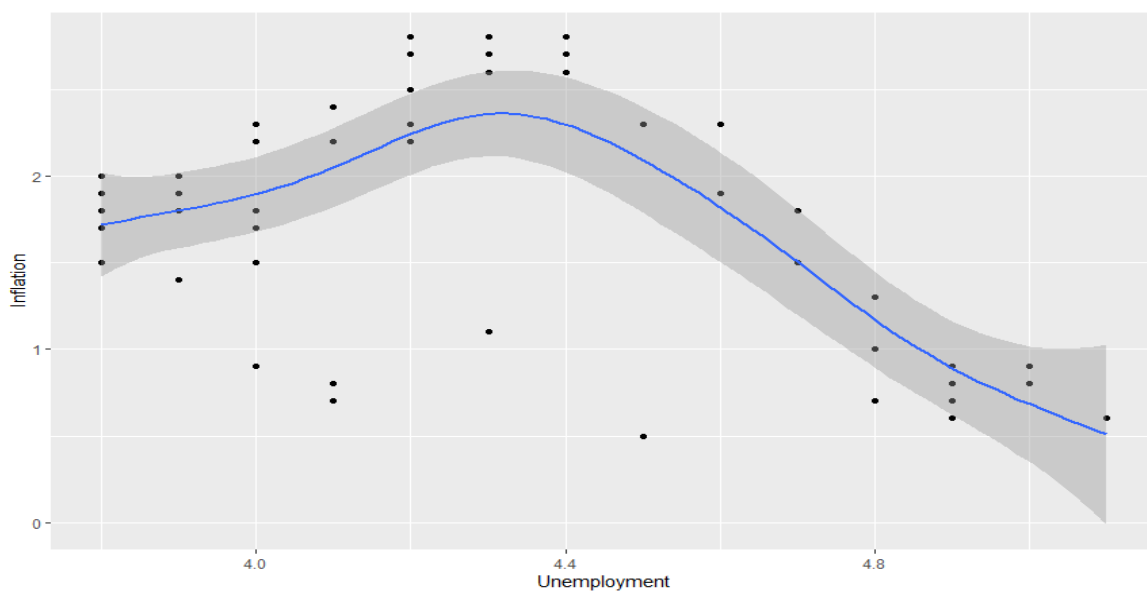
Figure 4. Smooth function of UK fitted using GAM.
