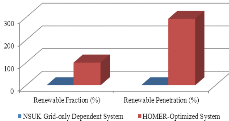
Fig. 9. Renewable profile
