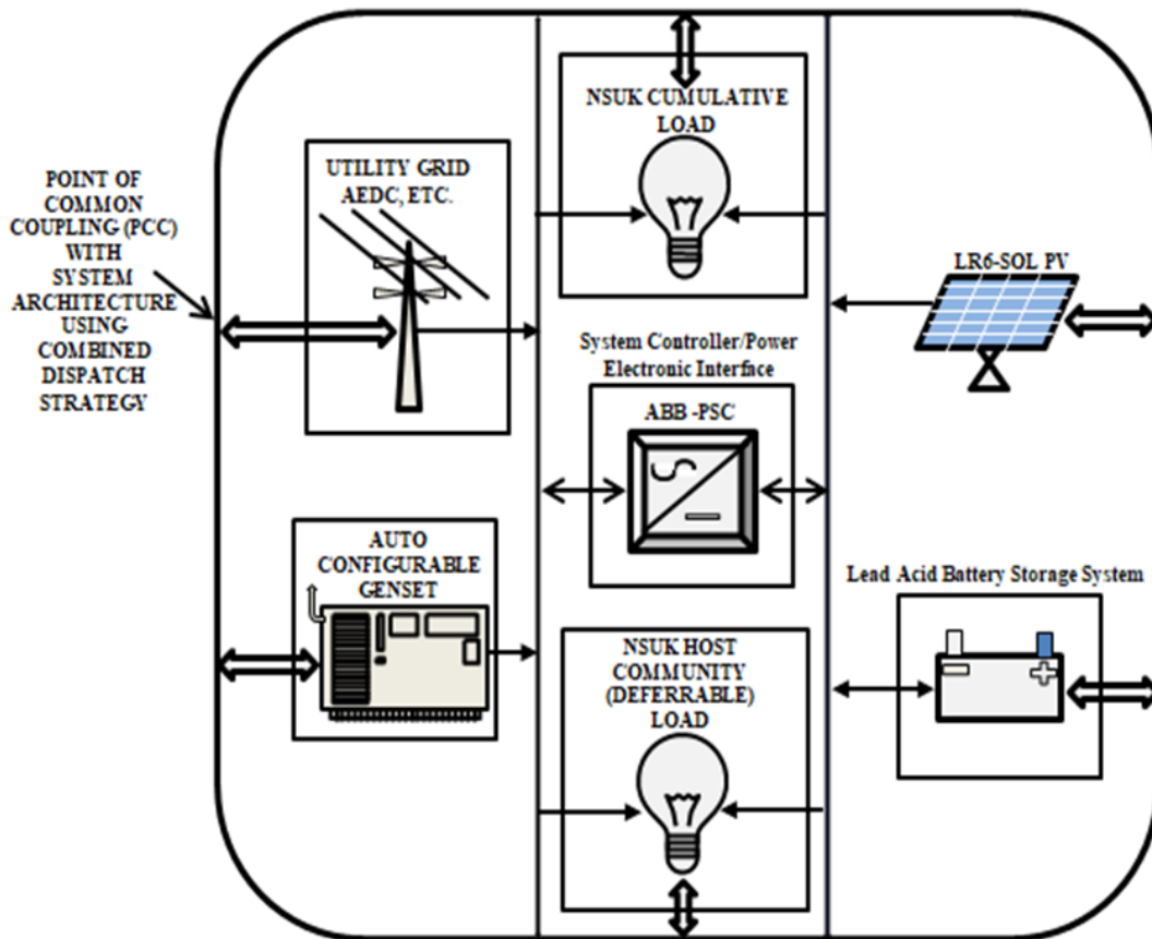
Fig. 11. Block diagram of the proposed micro grid system
