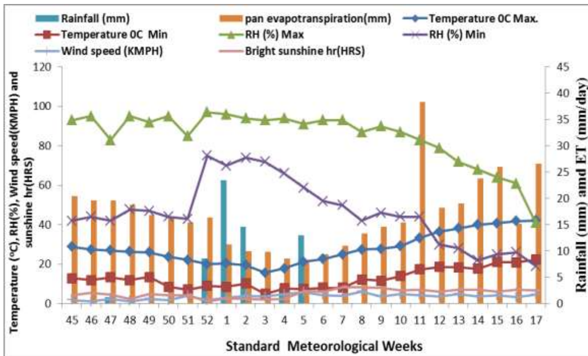
Fig. 2. Details of weather data during crop season (2021-22)
