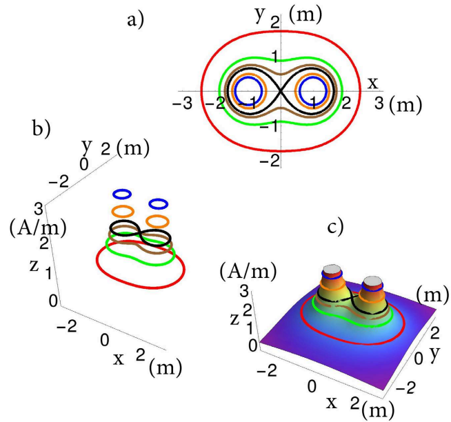
Figure 3. Three views of field curves around two parallel electrical-current wires with one (A) for both wires in the z direction. They are placed at xy (-1, 0) or (+1, 0) . In (a), (b) and (c), blue circles are nearest to one of each electrical-current wires with a field of 3.0 (A/m). When distances are larger, the field decreases until the current field curves are around both electrical wires. In between, and as in (b) and (c), black lines forming a horizontal number 8, show a pass between the two electrical wires exactly like a pass in a topographic level map between two mountains [14]. Only the black curve cut itself ((a)-(c)).
