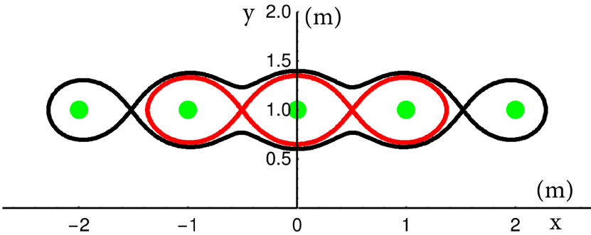
Figure 9. Pass between five identical and parallel current wires periodically placed and aligned ( y = 1 ) with inter-distance of one (m) in x direction. Green points show positions of the five wires, and seven domains are formed. The red field curve at 5.73295 A/m has two passes as for the black field curve which is at 5.345208 A/m.
