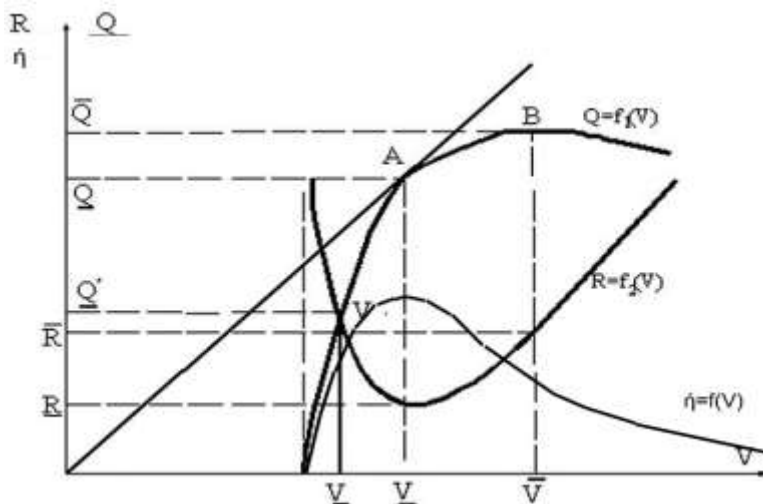
Fig. 2. Characteristic dependences of the parameters of gas-lift wells
