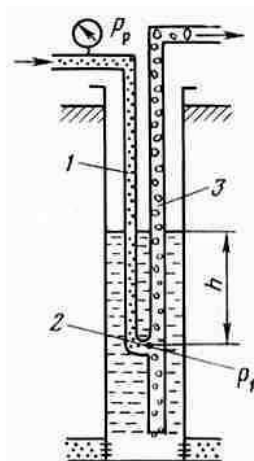
Fig. 1. Schematic diagram of a gas lift
