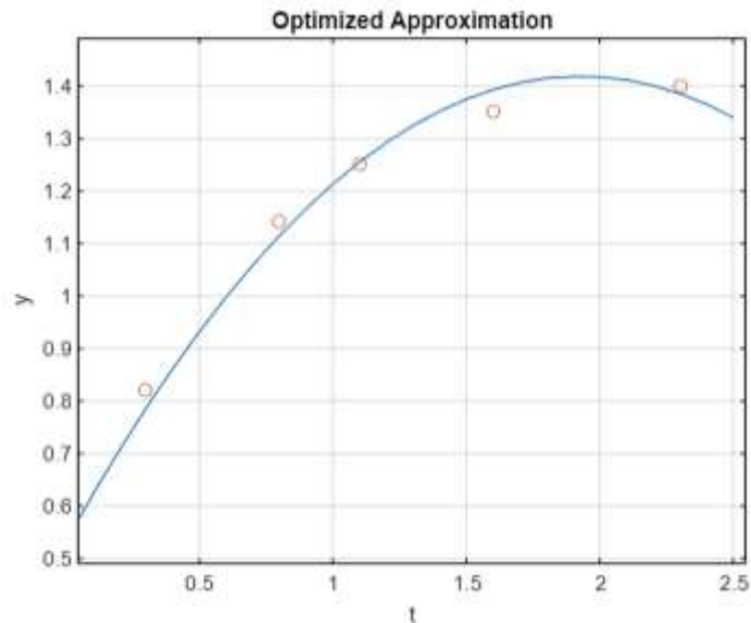
Fig. 4. Optimization approximation
