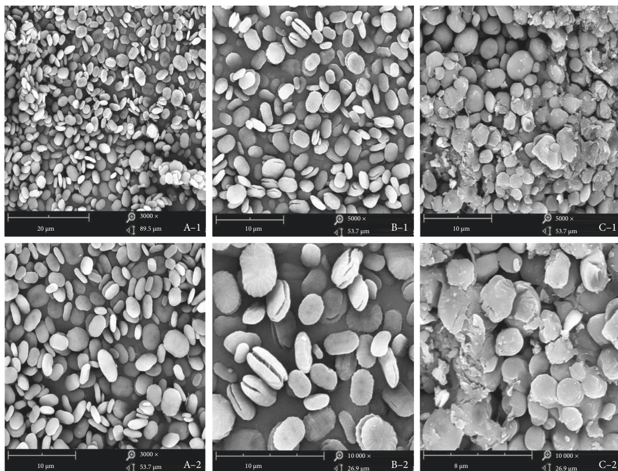
FIGURE 2: SEM images of samples. (A-1, A-2) EGP, (B-1, B-2) H-EGP, and (C-1, C-2) C-EGP.
